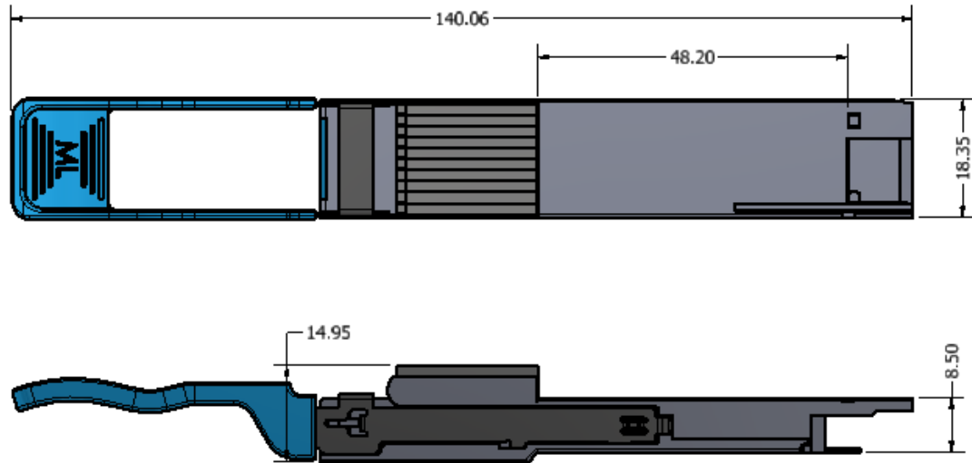
Figure 11: Mechanical Dimensions
